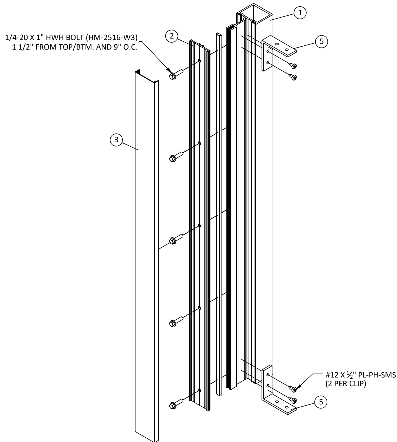
4518 STACKING MULL ASSEMBLY TYPICAL
